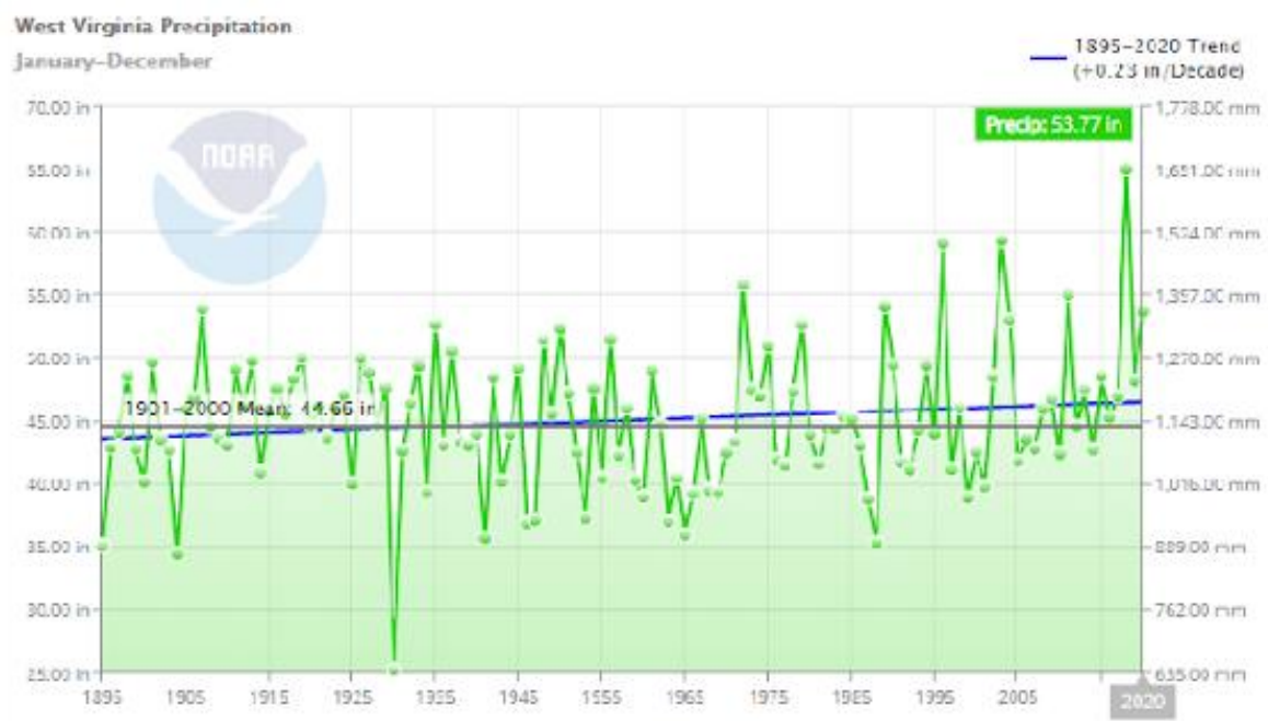
Figure 1. WV's annual precipitation from 1895 – 2020 ( from National Oceanic and Atmospheric Administration ).
