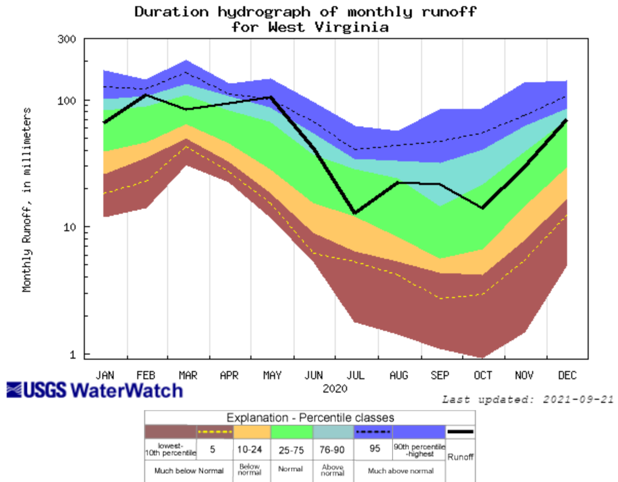
Figure 9. WV 2020 monthly hydrograph. Note logarithmic scale ( from USGS ).
