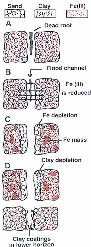
Figure 8. Schematic illustration showing the formation of redox depletions. The process begins with: (A) a decomposing root lying in a channel. When the channel fills with water (B), Fe in soil along the channel is reduced when the root's decomposition occurs anaerobically. The reduced Fe (II) may diffuse into the soil matrix. An Fe depletion occurs along the channel when enough Fe has been lost to produce a color chroma of 2 or less. (C) Iron masses form when the Fe (II) in the matrix oxidizes to Fe (III). The loss of Fe makes clay along the channel dispersible, and water moving along the channel may illuviate this clay to a lower horizon. (D) Clay depletions form where the clay has been removed.
