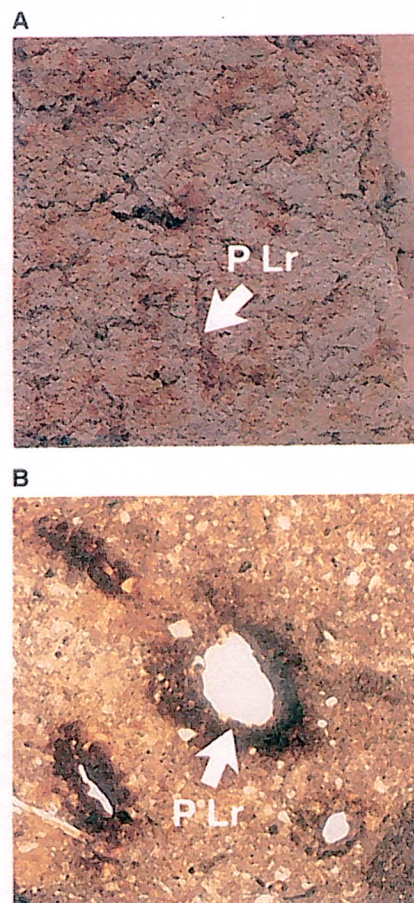
Figure 5. Examples of pore linings. Pore linings in (A) primarily are along root channels (PLr). (Photograph supplied by M. C. Rabenhorst). Pore linings are usually thin and can be difficult to see. In (B) a thin section shows black pore linings around root channels that are approximately 1 mm in diameter (photograph supplied by L. P. Wilding).
