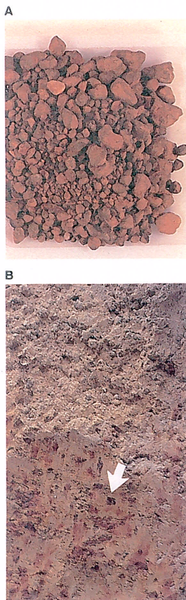
Figure 3. Examples of Fe/Mn nodules that have been washed (A) and as they appear in a pit wall (B). In (A) largest nodules are 20 mm in diameter. In (B) arrow shows a nodule also 20 mm in diameter.
