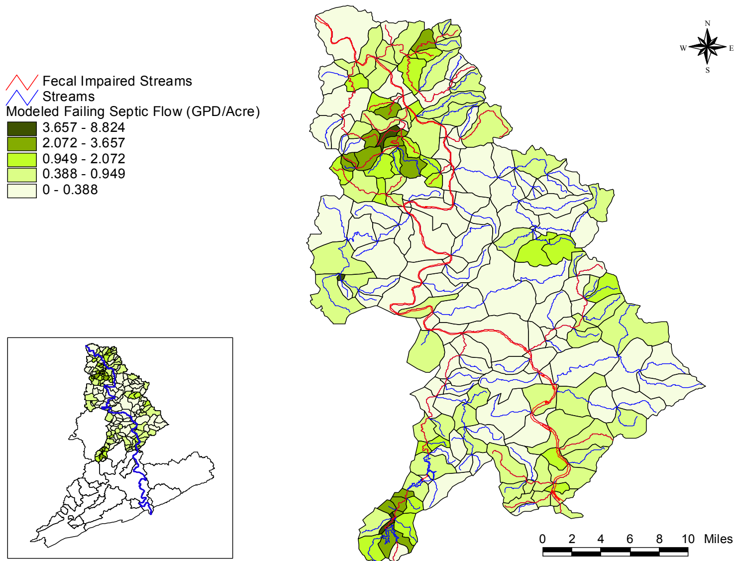
Figure A-1-3. Graphical representation of failing septic system flows in the Lower New River watershed
